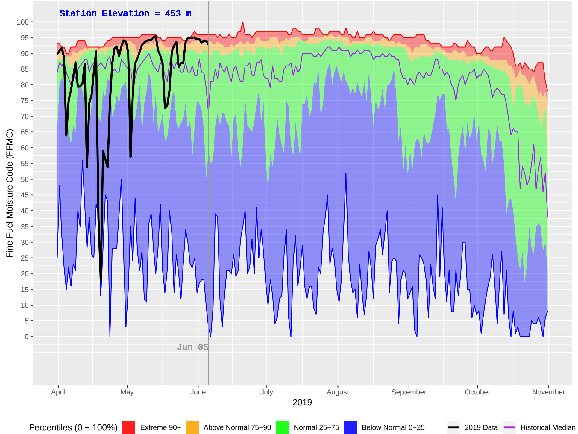
CLEARWATER HUB (239) : Historical (1976–2018) and Current (2019) Daily Fine Fuel Moisture Code (FFMC)
