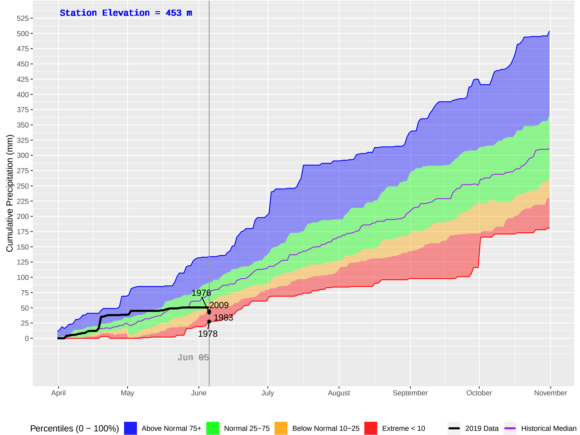
CLEARWATER HUB (239) : Historical (1976–2018), Current (2019) Daily Cumulative Precipitation
