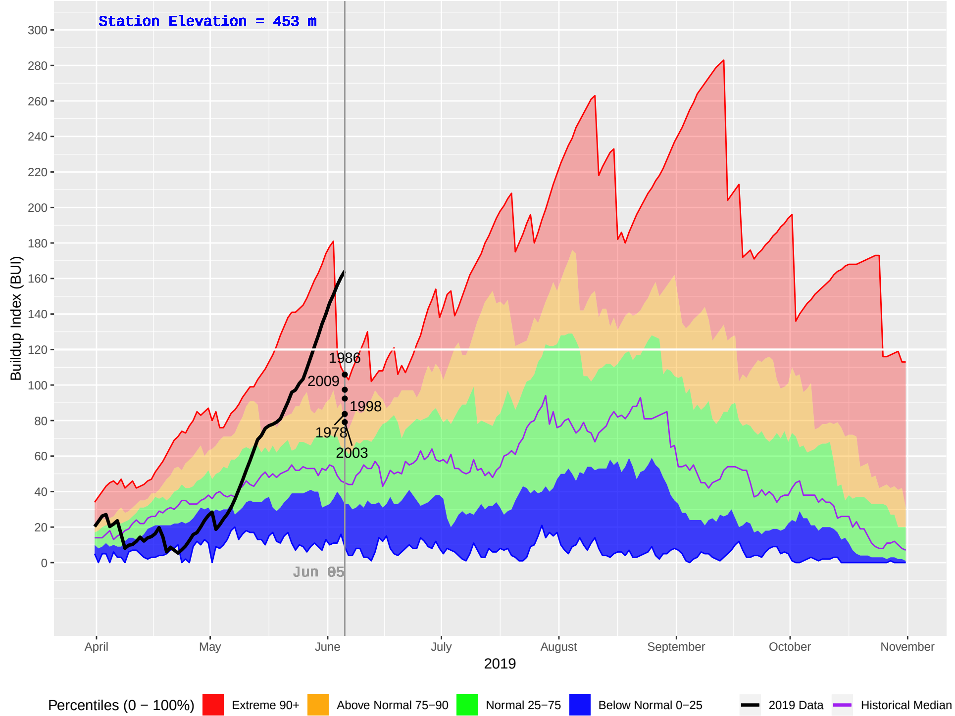
CLEARWATER HUB (239) : Historical (1976–2018), Current (2019) Daily Buildup Index (BUI)
