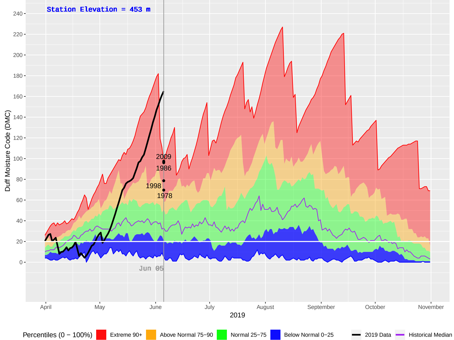
CLEARWATER HUB (239) : Historical (1976–2018), Current (2019) Daily Duff Moisture Code (DMC)
