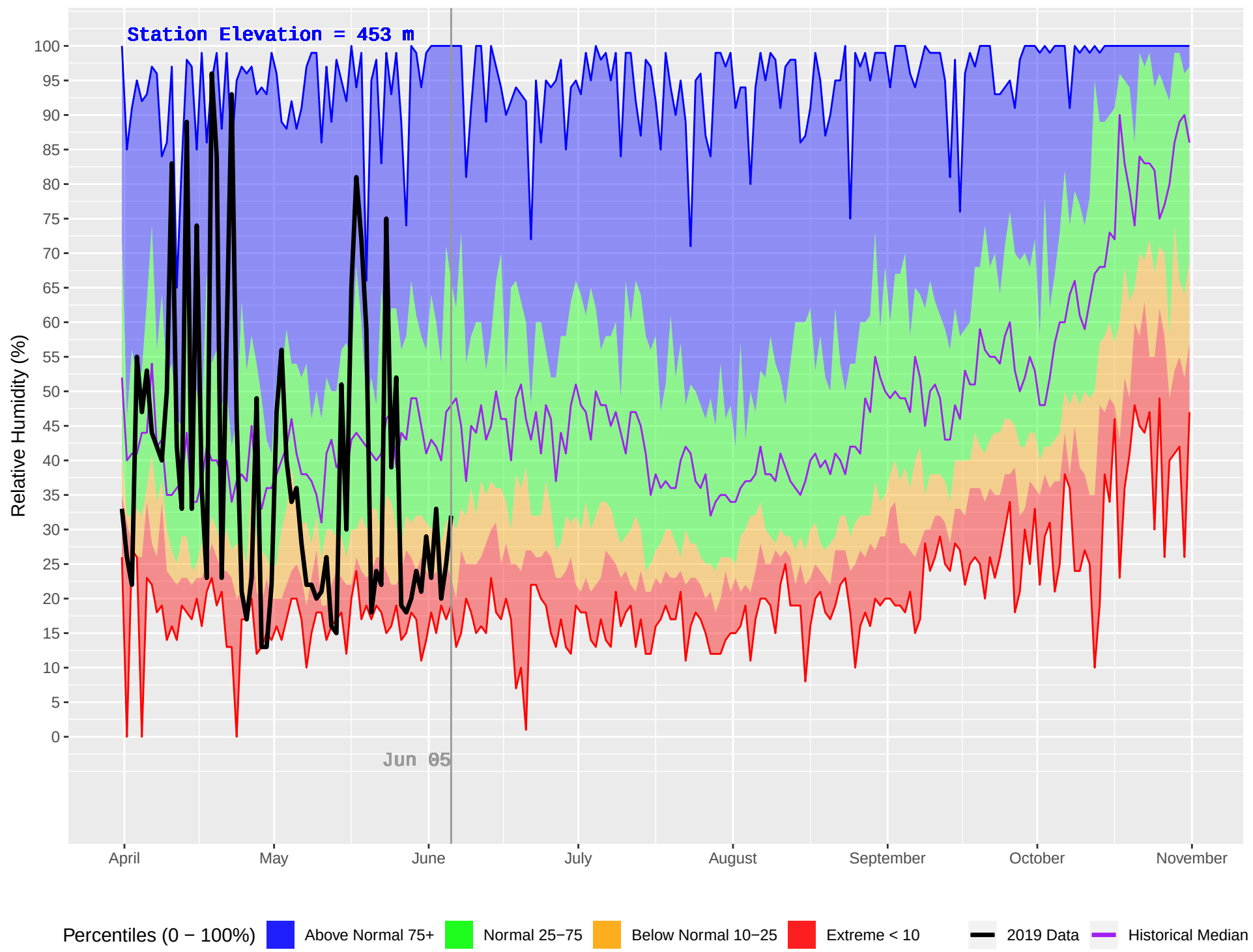
CLEARWATER HUB (239) : Historical (1976–2018) and Current (2019) Daily Relative Humidity
